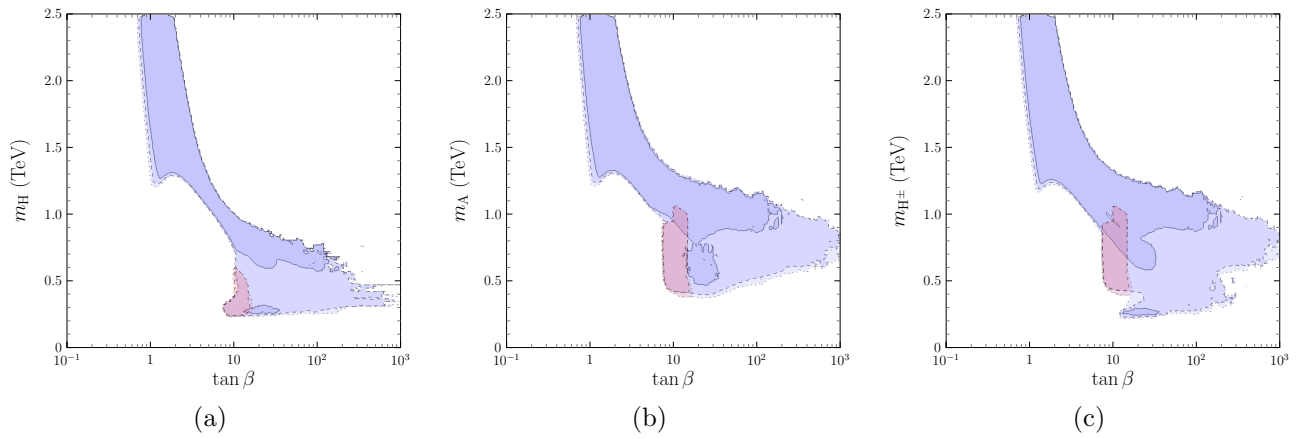
Figure 5: Masses vs. \tan\beta
