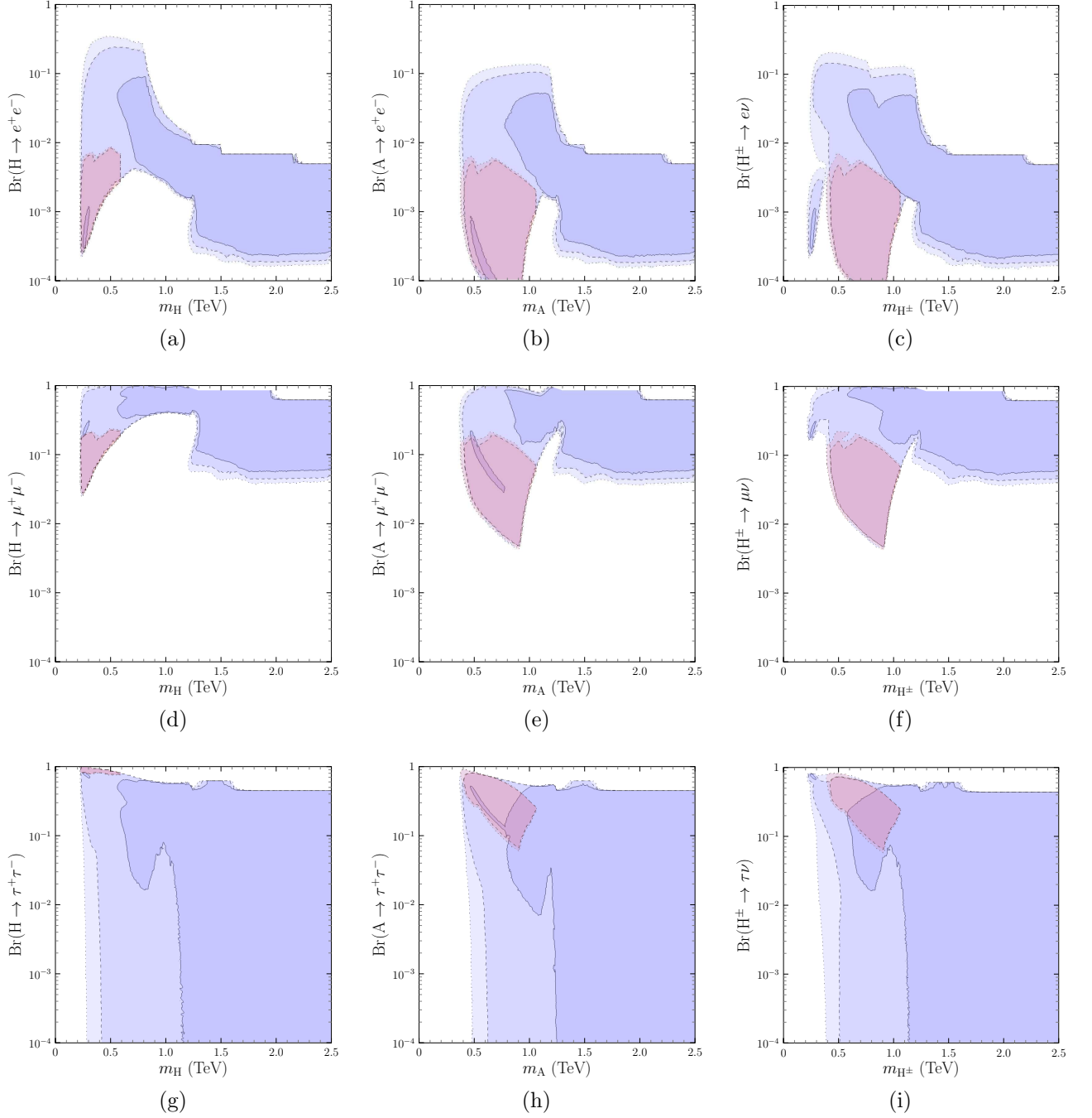
Figure 6: BR's of scalars (1)
