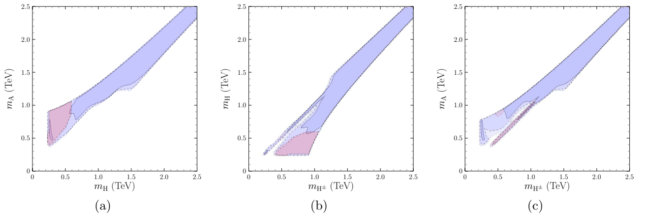
Figure 2: Scalar masses
