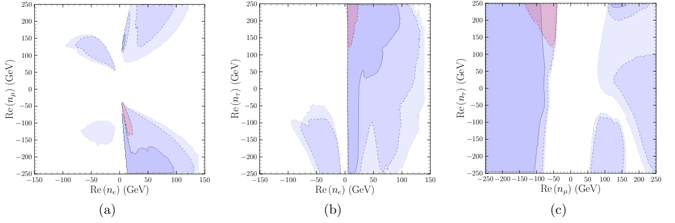
Figure 1: \text{Re}(n_\ell)
