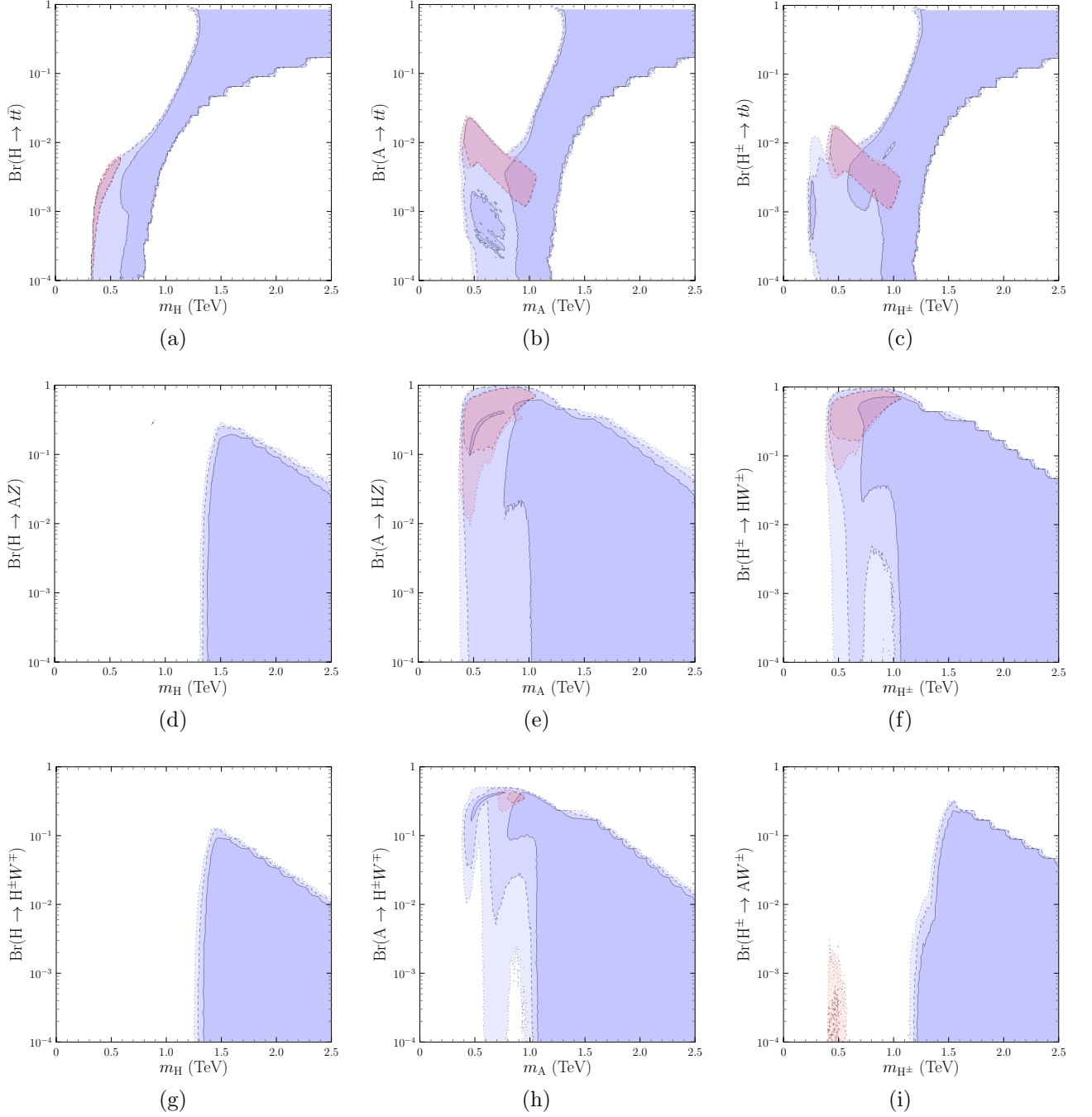
Figure 7: BR's of scalars (2)
