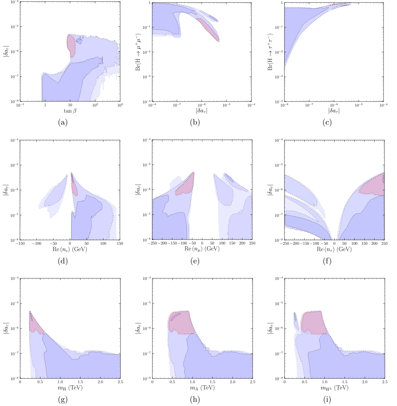
Figure 10: \delta a_\tau
