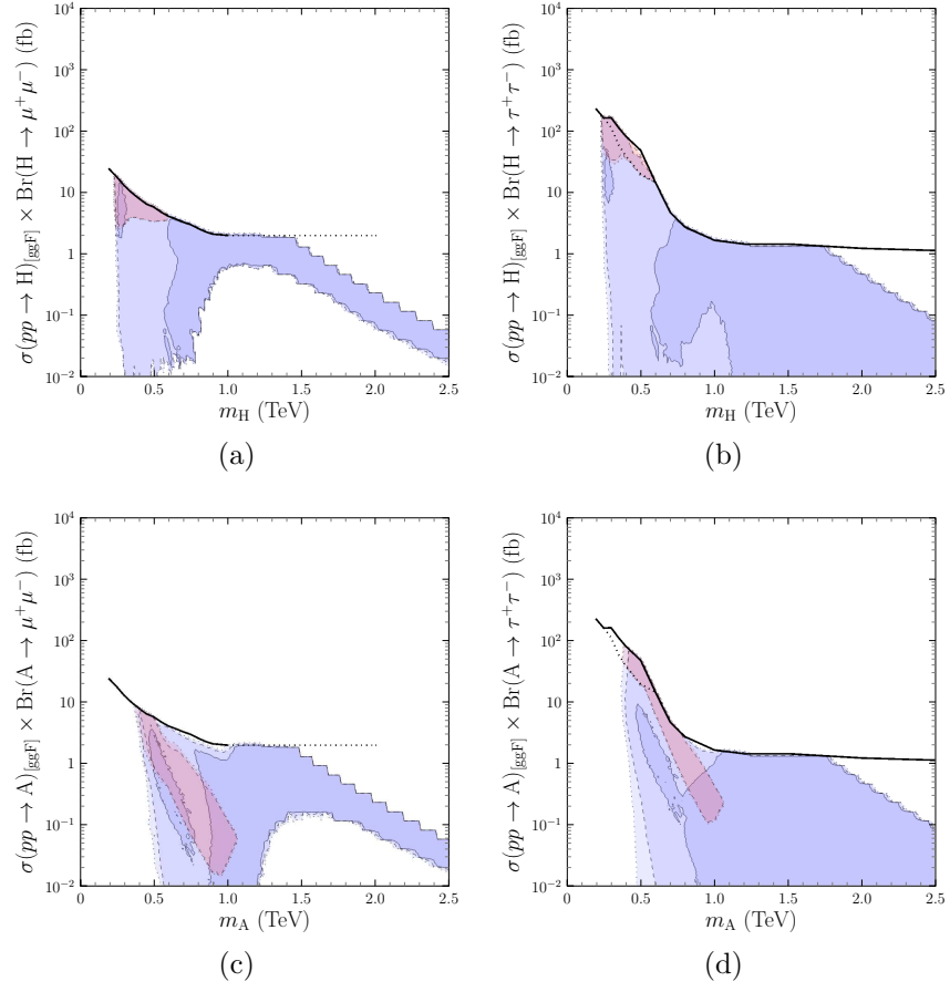
Figure 8: [pp]_{\text{ggF}} \rightarrow S \rightarrow \ell^+ \ell^-
