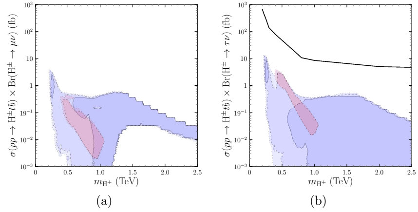
Figure 9: [pp] \rightarrow H^\pm(tb) \rightarrow \ell \nu
