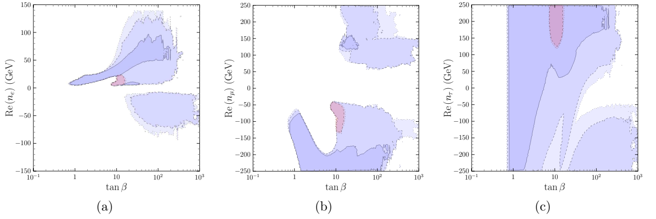
Figure 4: \text{Re}(n_\ell) vs. \tan\beta
