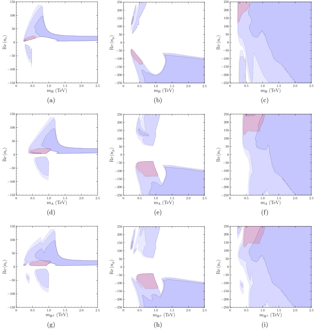
Figure 3: \text{Re}(n_\ell) vs Masses
