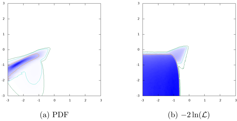
Figure 30: \log_{10} \sigma(pp \rightarrow H^\pm tb)(H^\pm \rightarrow HW^\pm) (fb) vs. \log_{10} \sigma(pp \rightarrow H^\pm tb)(H^\pm \rightarrow \tau^\pm \nu) (fb)
