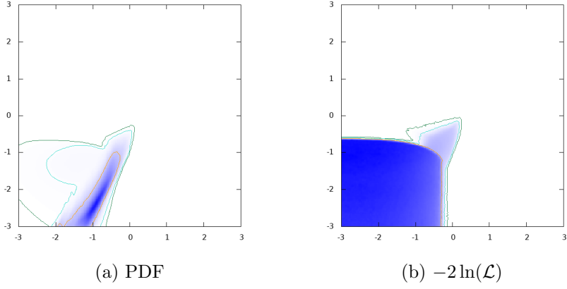
Figure 41: \log_{10} \sigma(pp \rightarrow H^\pm tb)(H^\pm \rightarrow \tau^\pm \nu) (fb) vs. \log_{10} \sigma(pp \rightarrow H^\pm tb)(H^\pm \rightarrow HW^\pm) (fb)
