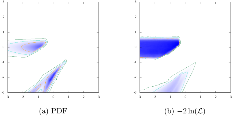
Figure 29: \log_{10} \sigma(pp \rightarrow H^\pm tb)(H^\pm \rightarrow tb) (fb) vs. \log_{10} \sigma(pp \rightarrow H^\pm tb)(H^\pm \rightarrow \tau^\pm \nu) (fb)
