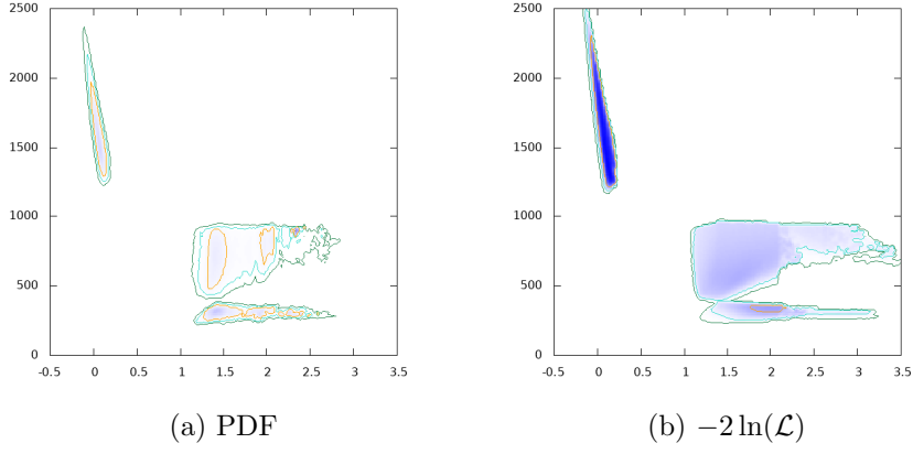
Figure 1: m_{H^\pm} GeV vs. \log_{10} \tan \beta
