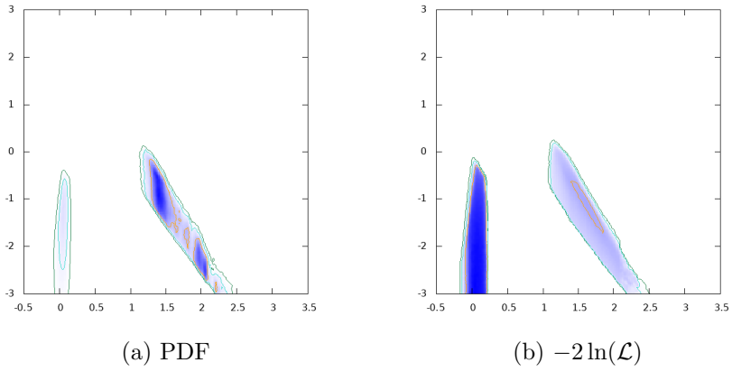
Figure 6: \log_{10} \sigma(pp \rightarrow H^\pm tb)(H^\pm \rightarrow HW^\pm) (fb) vs. \log_{10} \tan \beta
