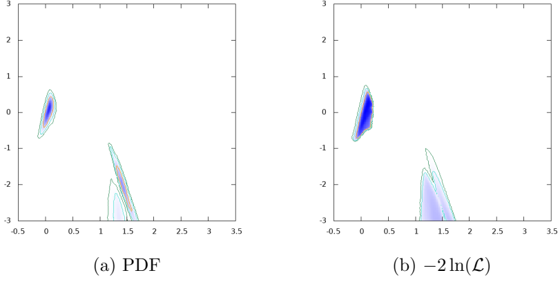
Figure 5: \log_{10} \sigma(pp \rightarrow H^\pm tb)(H^\pm \rightarrow tb) (fb) vs. \log_{10} \tan \beta
