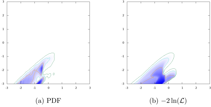
Figure 21: \log_{10} \sigma(pp \rightarrow H^\pm tb)(H^\pm \rightarrow e^\pm \nu) (fb) vs. \log_{10} \sigma(pp \rightarrow H^\pm tb)(H^\pm \rightarrow \mu^\pm \nu) (fb)
