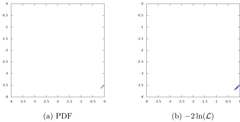
Figure 51: \log_{10}\text{BR}(H \rightarrow \bar{b}b) vs. \log_{10}\text{BR}(H \rightarrow t\bar{t})
