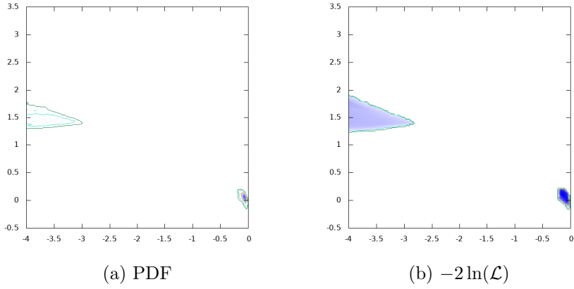
Figure 46: \log_{10} \tan \beta vs. \log_{10} \text{BR}(H \rightarrow t\bar{t})
