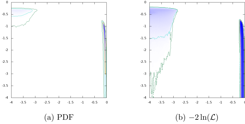
Figure 50: \log_{10}\text{BR}(H \rightarrow \tau^+\tau^-) vs. \log_{10}\text{BR}(H \rightarrow t\bar{t})
