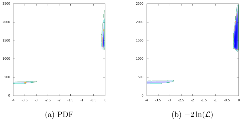
Figure 47: m_H GeV vs. \log_{10} \text{BR}(H \rightarrow t\bar{t})
