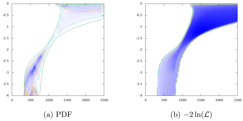
Figure 16: \log_{10}\text{BR}(H \rightarrow t\bar{t}) vs. m_H GeV
