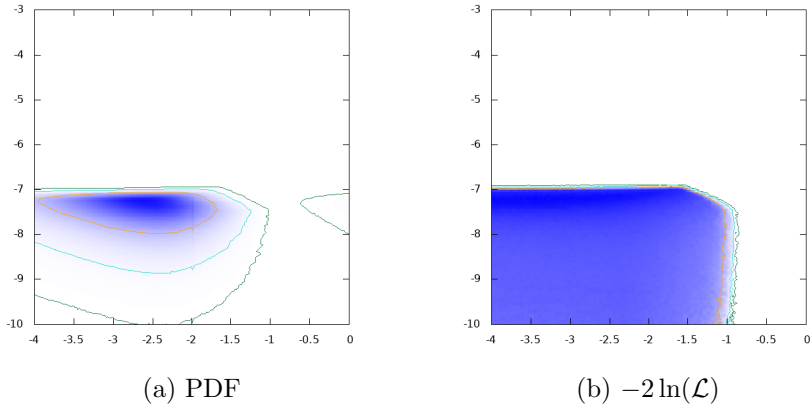
Figure 93: \log_{10}|\delta a_\tau| vs. \log_{10}\text{BR}(H \rightarrow H^\pm W^\mp)
