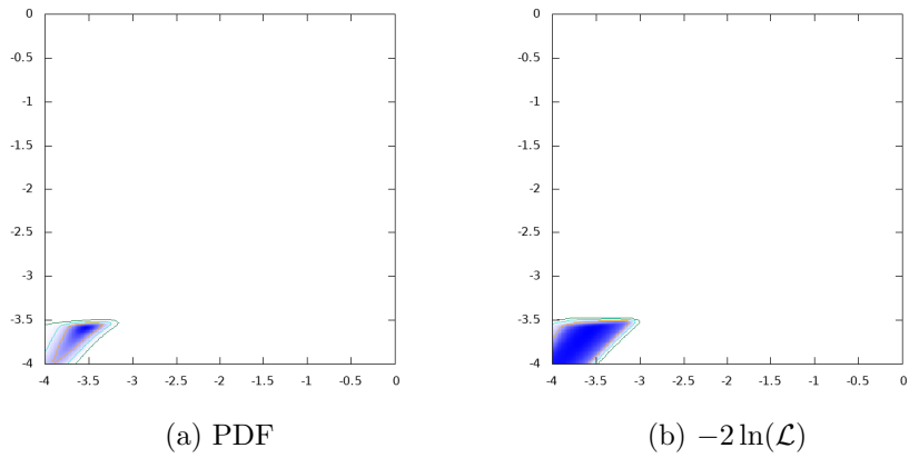
Figure 108: \log_{10}\text{BR}(H \rightarrow \bar{b}b) vs. \log_{10}\text{BR}(H \rightarrow SS)
