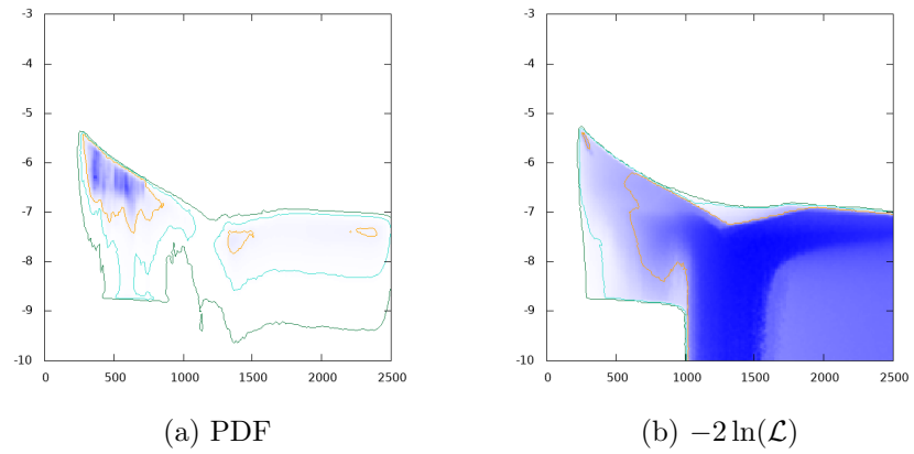
Figure 12: \log_{10} |\delta a_\tau| vs. m_H GeV
