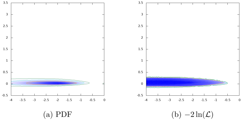
Figure 81: \log_{10} \tan \beta vs. \log_{10} \text{BR}(H \rightarrow AZ)
