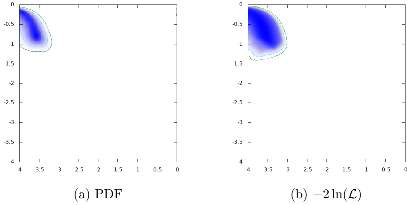
Figure 105: \log_{10}\text{BR}(H \rightarrow \mu^+\mu^-) vs. \log_{10}\text{BR}(H \rightarrow SS)
