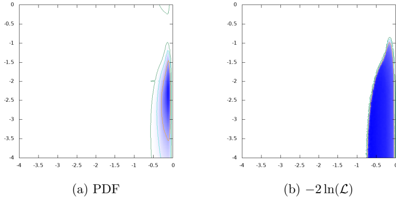
Figure 69: \log_{10}\text{BR}(H \rightarrow H^\pm W^\mp) vs. \log_{10}\text{BR}(H \rightarrow \bar{t}t)
