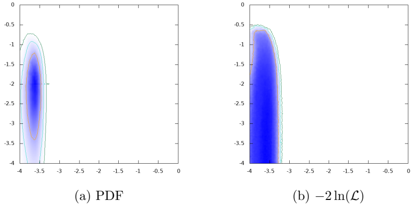
Figure 109: \log_{10}\text{BR}(H \rightarrow AZ) vs. \log_{10}\text{BR}(H \rightarrow SS)
