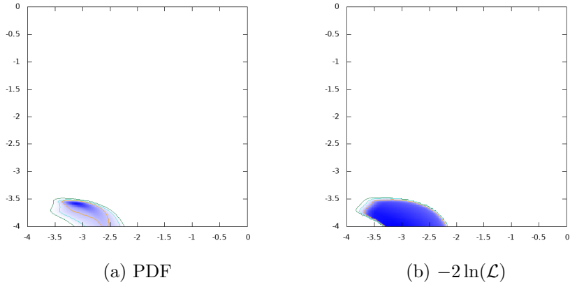
Figure 37: \log_{10}\text{BR}(H \rightarrow \bar{b}b) vs. \log_{10}\text{BR}(H \rightarrow e^+e^-)
