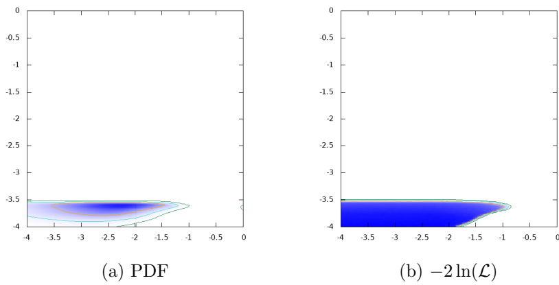
Figure 98: \log_{10}\text{BR}(H \rightarrow b\bar{b}) vs. \log_{10}\text{BR}(H \rightarrow H^\pm W^\mp)
