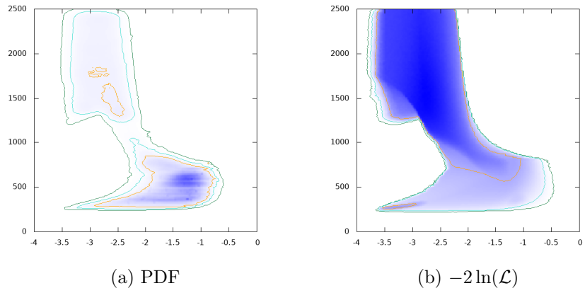
Figure 32: m_H GeV vs. \log_{10} \text{BR}(H \rightarrow e^+e^-)
