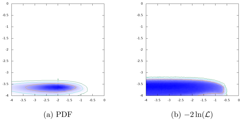
Figure 90: \log_{10}\text{BR}(H \rightarrow SS) vs. \log_{10}\text{BR}(H \rightarrow AZ)
