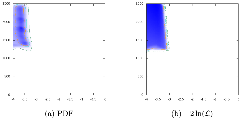
Figure 102: m_H GeV vs. \log_{10} \text{BR}(H \rightarrow SS)
