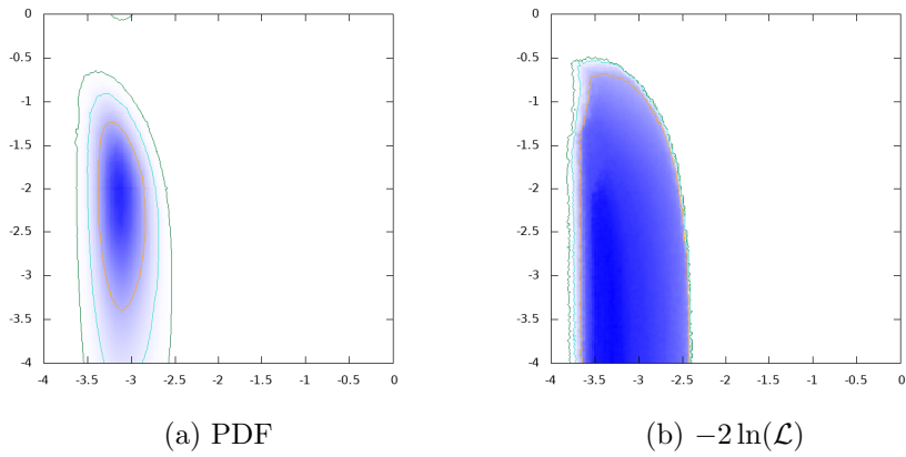
Figure 38: \log_{10}\text{BR}(H \rightarrow AZ) vs. \log_{10}\text{BR}(H \rightarrow e^+e^-)
