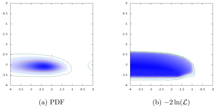
Figure 94: \log_{10}\text{BR}(H \rightarrow e^+ e^-) vs. \log_{10}\text{BR}(H \rightarrow H^\pm W^\mp)
