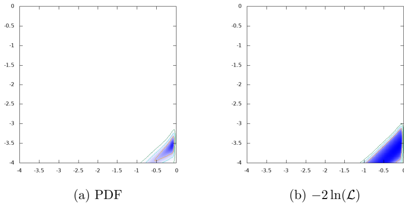
Figure 70: \log_{10}\text{BR}(H \rightarrow SS) vs. \log_{10}\text{BR}(H \rightarrow \bar{t}t)
