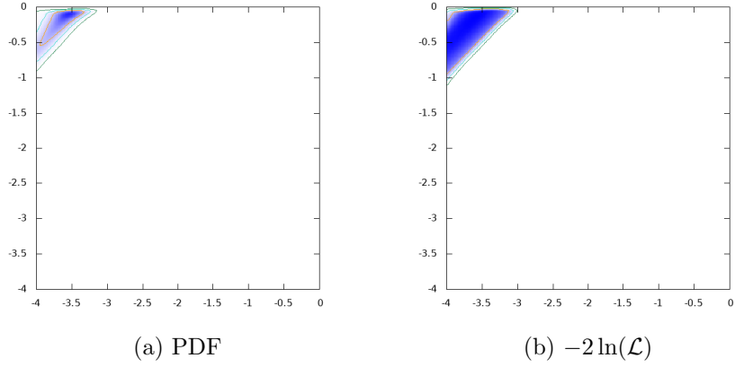
Figure 107: \log_{10}\text{BR}(H \rightarrow \bar{t}t) vs. \log_{10}\text{BR}(H \rightarrow SS)
