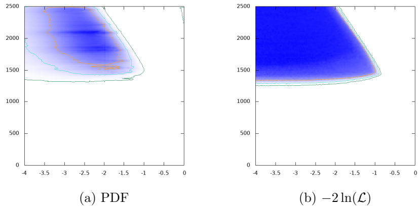
Figure 92: m_H GeV vs. \log_{10} \text{BR}(H \rightarrow H^\pm W^\mp)
