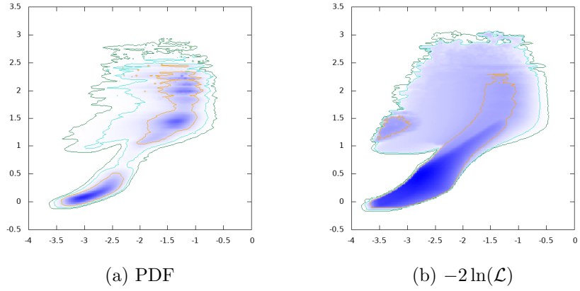
Figure 31: \log_{10} \tan \beta vs. \log_{10} \text{BR}(H \rightarrow e^+e^-)
