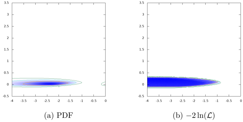
Figure 91: \log_{10} \tan \beta vs. \log_{10} \text{BR}(H \rightarrow H^\pm W^\mp)
