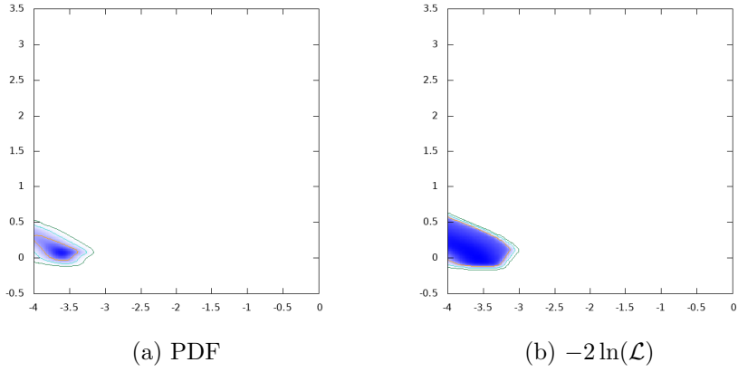
Figure 101: \log_{10} \tan \beta vs. \log_{10} \text{BR}(H \rightarrow SS)
