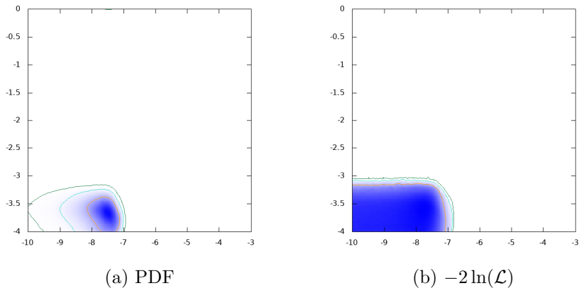
Figure 30: \log_{10}\text{BR}(H \rightarrow SS) vs. \log_{10}|\delta a_\tau|
