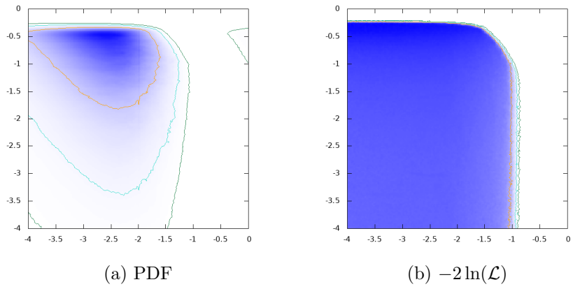
Figure 96: \log_{10}\text{BR}(H \rightarrow \tau^+\tau^-) vs. \log_{10}\text{BR}(H \rightarrow H^\pm W^\mp)
