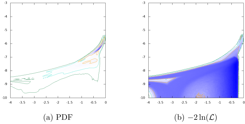
Figure 53: \log_{10}|\delta a_\tau| vs. \log_{10}\text{BR}(H \rightarrow \tau^+\tau^-)
