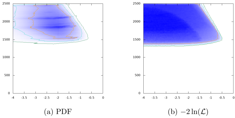
Figure 82: m_H GeV vs. \log_{10} \text{BR}(H \rightarrow AZ)
