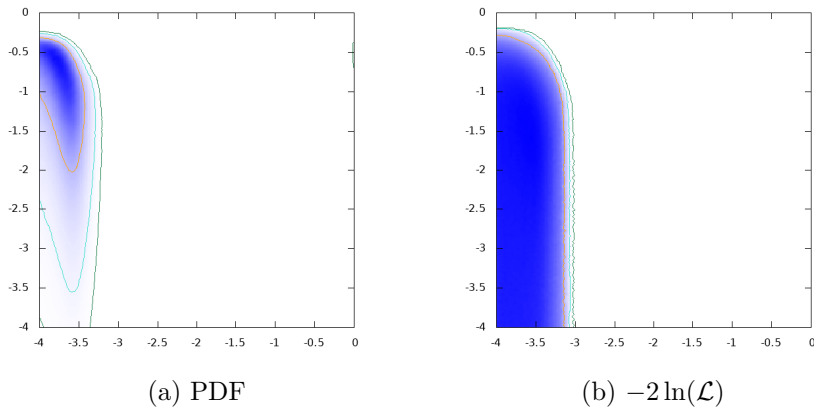
Figure 106: \log_{10}\text{BR}(H \rightarrow \tau^+\tau^-) vs. \log_{10}\text{BR}(H \rightarrow SS)
