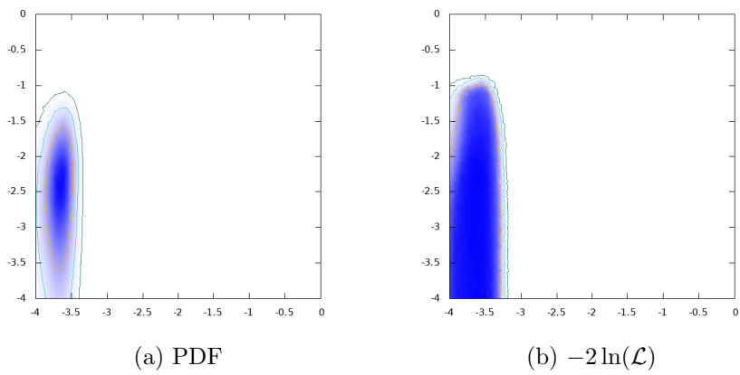
Figure 110: \log_{10}\text{BR}(H \rightarrow H^\pm W^\mp) vs. \log_{10}\text{BR}(H \rightarrow SS)
