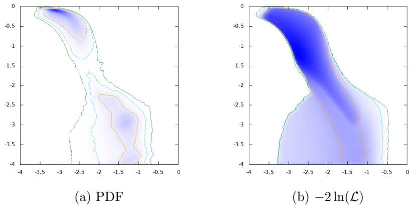
Figure 36: \log_{10}\text{BR}(H \rightarrow t\bar{t}) vs. \log_{10}\text{BR}(H \rightarrow e^+e^-)
