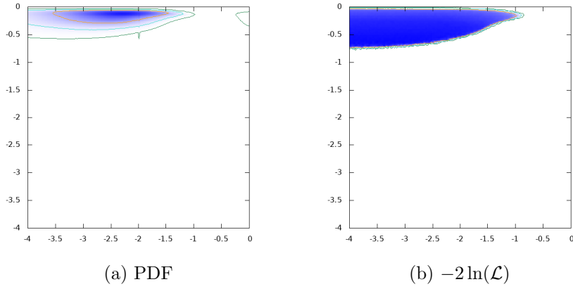
Figure 97: \log_{10}\text{BR}(H \rightarrow t\bar{t}) vs. \log_{10}\text{BR}(H \rightarrow H^\pm W^\mp)
