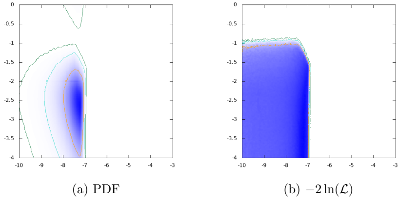
Figure 29: \log_{10}\text{BR}(H \rightarrow H^\pm W^\mp) vs. \log_{10}|\delta a_\tau|
