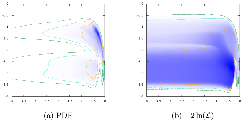
Figure 54: \log_{10}\text{BR}(H \rightarrow e^+e^-) vs. \log_{10}\text{BR}(H \rightarrow \tau^+\tau^-)
