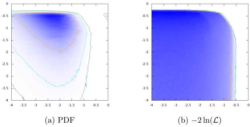
Figure 86: \log_{10}\text{BR}(H \rightarrow \tau^+\tau^-) vs. \log_{10}\text{BR}(H \rightarrow AZ)
