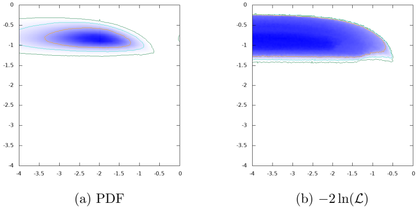
Figure 85: \log_{10}\text{BR}(H \rightarrow \mu^+\mu^-) vs. \log_{10}\text{BR}(H \rightarrow AZ)
