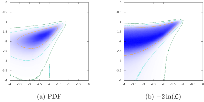
Figure 89: \log_{10}\text{BR}(H \rightarrow H^\pm W^\mp) vs. \log_{10}\text{BR}(H \rightarrow AZ)
