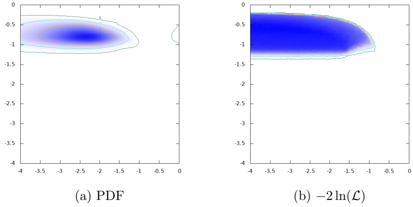
Figure 95: \log_{10}\text{BR}(H \rightarrow \mu^+\mu^-) vs. \log_{10}\text{BR}(H \rightarrow H^\pm W^\mp)
