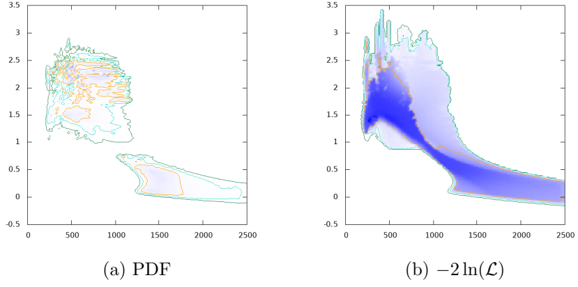
Figure 7: \log_{10} \tan \beta vs. m_{H^\pm} GeV
