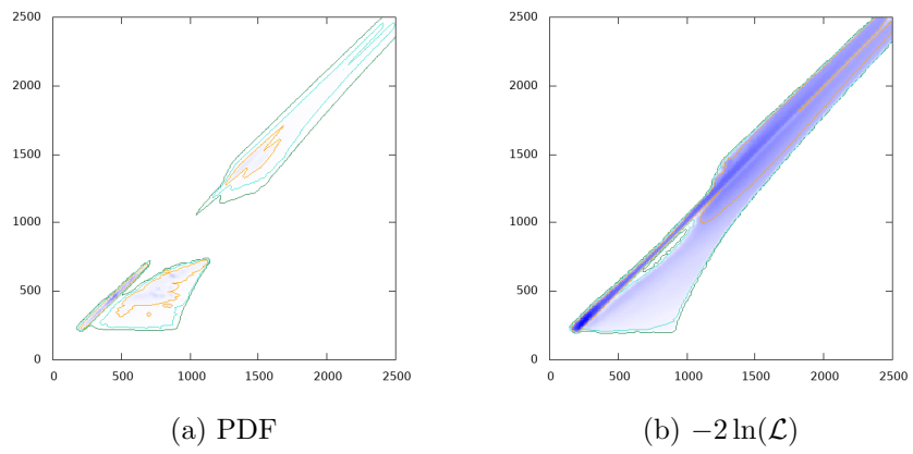
Figure 10: m_H GeV vs. m_{H^\pm} GeV
