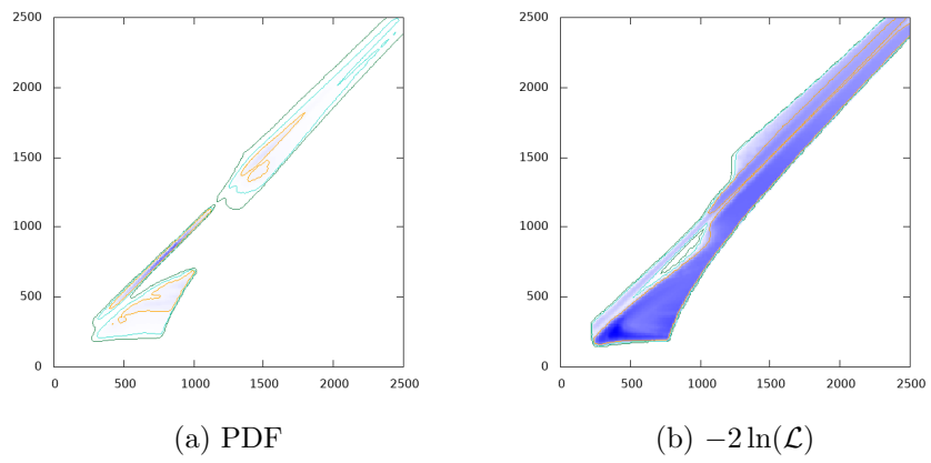
Figure 26: m_{H^\pm} GeV vs. m_A GeV
