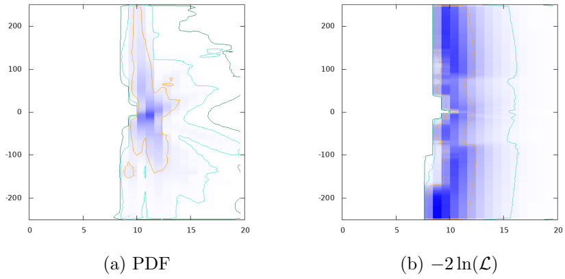
Figure 72: Re(n_\tau) vs. \chi^2(\text{tree Charged})
