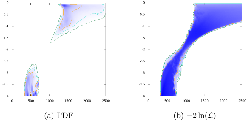
Figure 14: \log_{10}\text{BR}(H \rightarrow t\bar{t}) vs. m_H GeV
