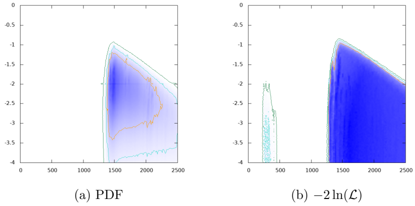
Figure 17: \log_{10}\text{BR}(H \rightarrow H^\pm W^\mp) vs. m_H GeV
