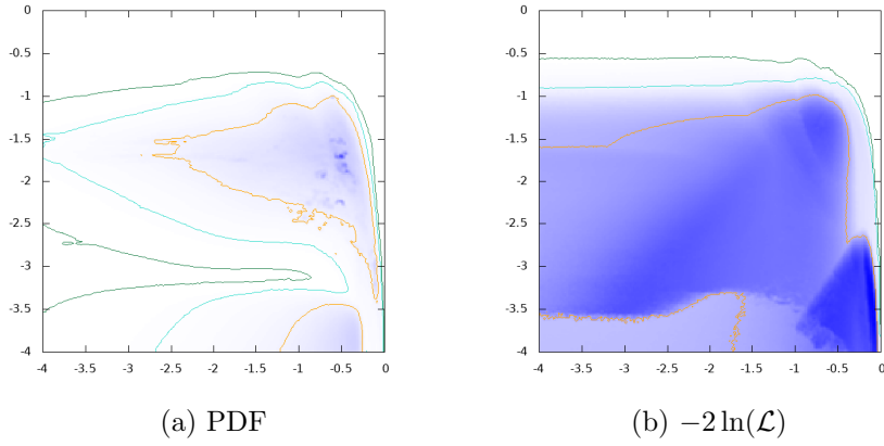
Figure 39: \log_{10}\text{BR}(H \rightarrow e^+e^-) vs. \log_{10}\text{BR}(H \rightarrow \tau^+\tau^-)
