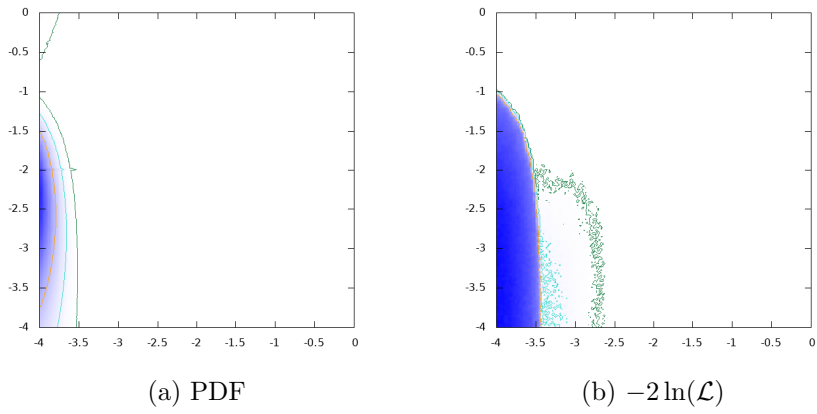
Figure 26: \log_{10}\text{BR}(H \rightarrow H^\pm W^\mp) vs. \log_{10}\text{BR}(H \rightarrow e^+e^-)
