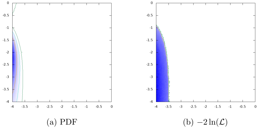
Figure 25: \log_{10}\text{BR}(H \rightarrow AZ) vs. \log_{10}\text{BR}(H \rightarrow e^+e^-)
