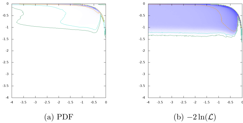
Figure 40: \log_{10}\text{BR}(H \rightarrow \mu^+\mu^-) vs. \log_{10}\text{BR}(H \rightarrow \tau^+\tau^-)
