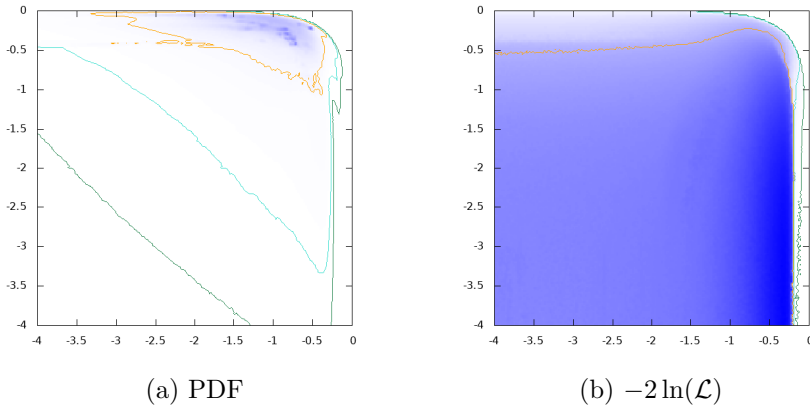
Figure 34: \log_{10}\text{BR}(H^\pm \rightarrow HW^\pm) vs. \log_{10}\text{BR}(H^\pm \rightarrow \tau^\pm \nu)
