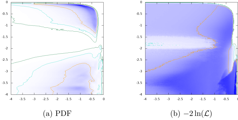
Figure 33: \log_{10}\text{BR}(H^\pm \rightarrow tb) vs. \log_{10}\text{BR}(H^\pm \rightarrow \tau^\pm \nu)
