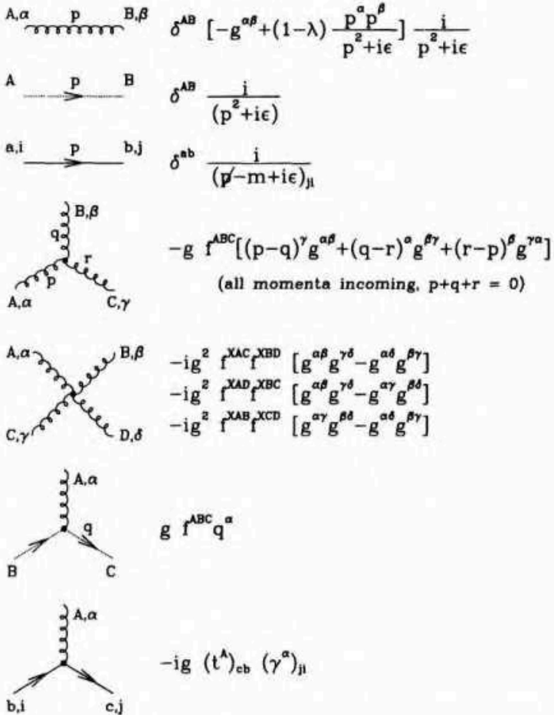
Fig. 1.3. Feynman rules for QCD in a covariant gauge for gluons (curly lines), fermions (solid lines) and ghosts (dotted lines).
